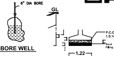
FOUNDATION DETAILS
