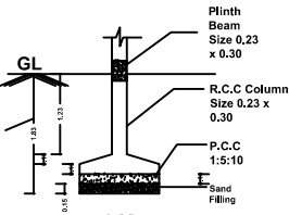
FOUNDATION DETAILS
