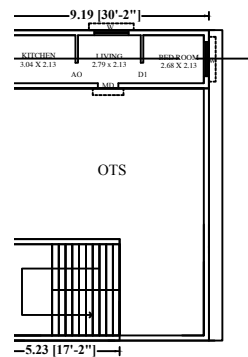
RO.FIRST FLOOR PLAN
