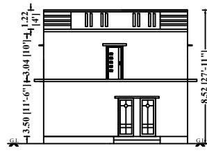
FRONT ELEVATION
