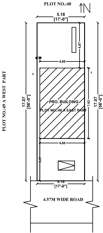
SITE PLAN
