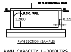
RWH_CAPACITY_L=2000LTRS
