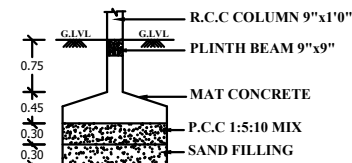
COLUMN FOUNDATION (NOT TO SCALE)
