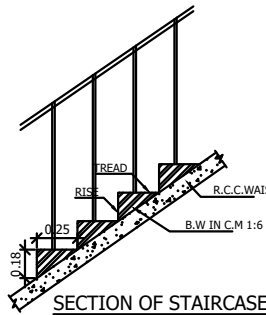
SECTION OF STAIRCASE (NOT TO SCALE)
