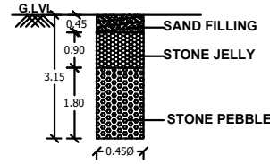
RAIN WATER HARVESTING PIT (NOT TO SCALE)
