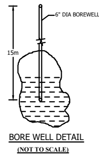
BORE WELL DETAIL (NOT TO SCALE)
