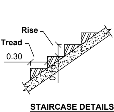
STAIRCASE DETAILS
