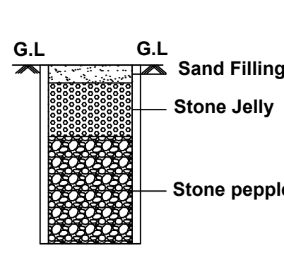
DETAILS OF RAIN WATER HARVESTING
