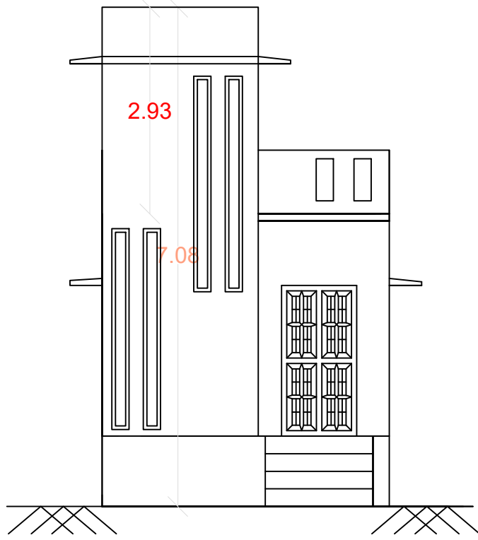
FRONT ELEVATION
