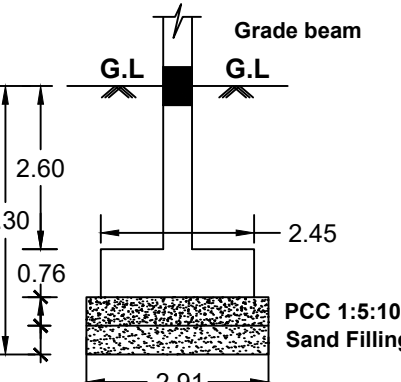
FOUNDATION DETAILS
