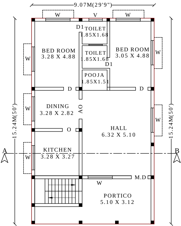
PRO.GROUND FLOOR PLAN (EAST FACING)
