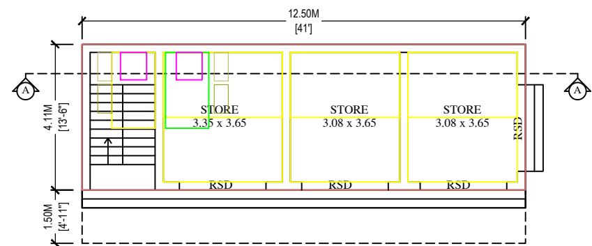
PRO.GROUND FLOOR PLAN
