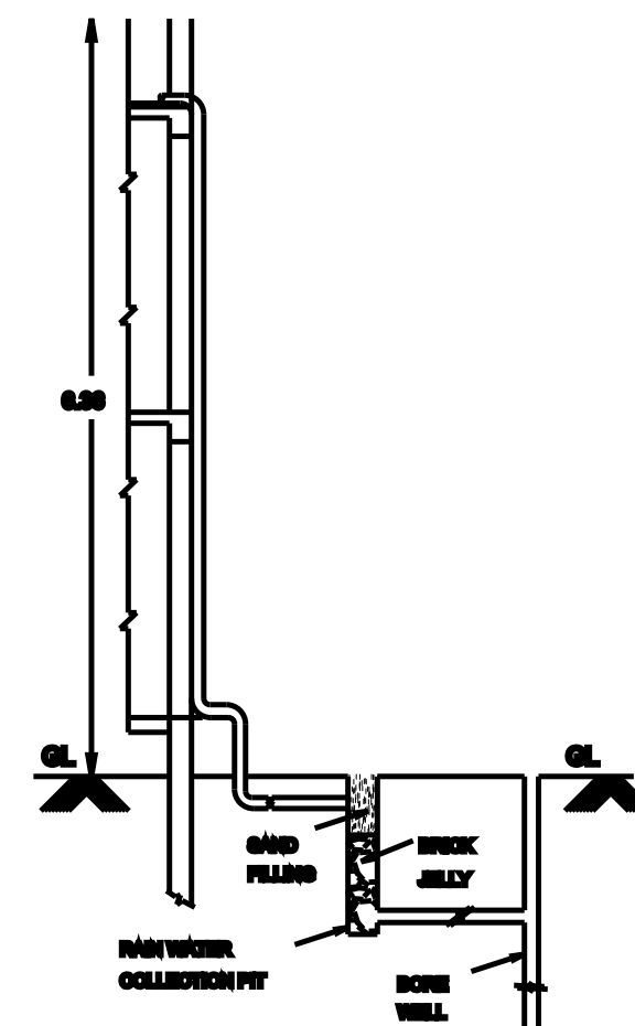
RAIN WATER HARVESTING SYSTEM RWH_CAPACITY_L=1000LTRS
