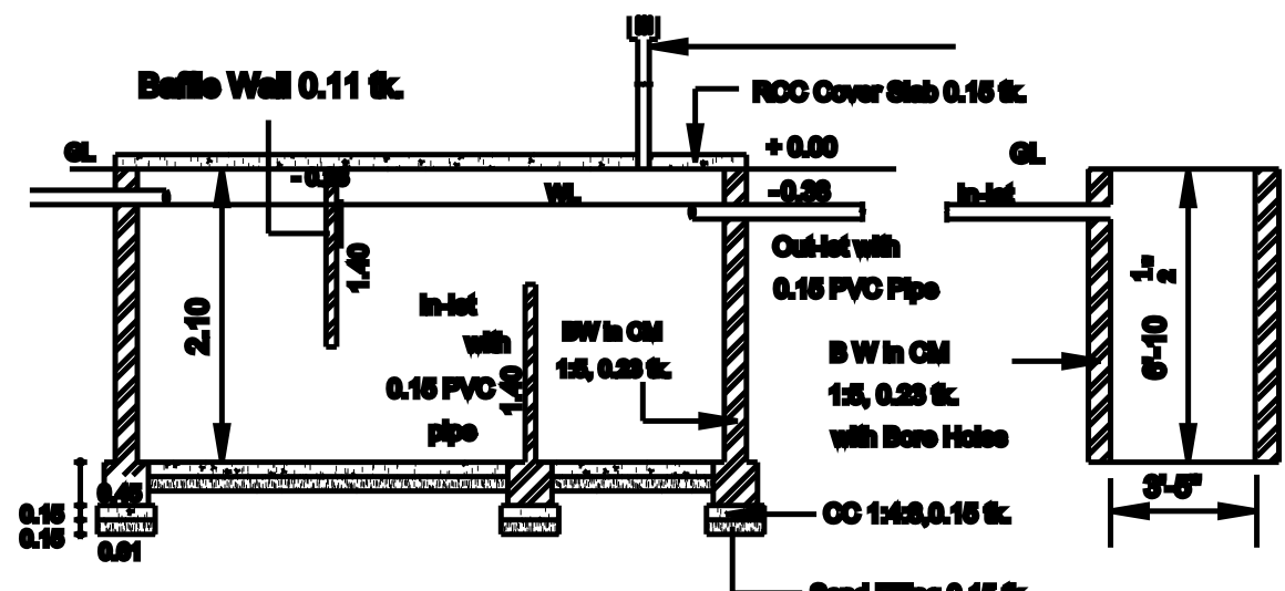
SECTION - SEPTIC TANK & SOAK PIT
