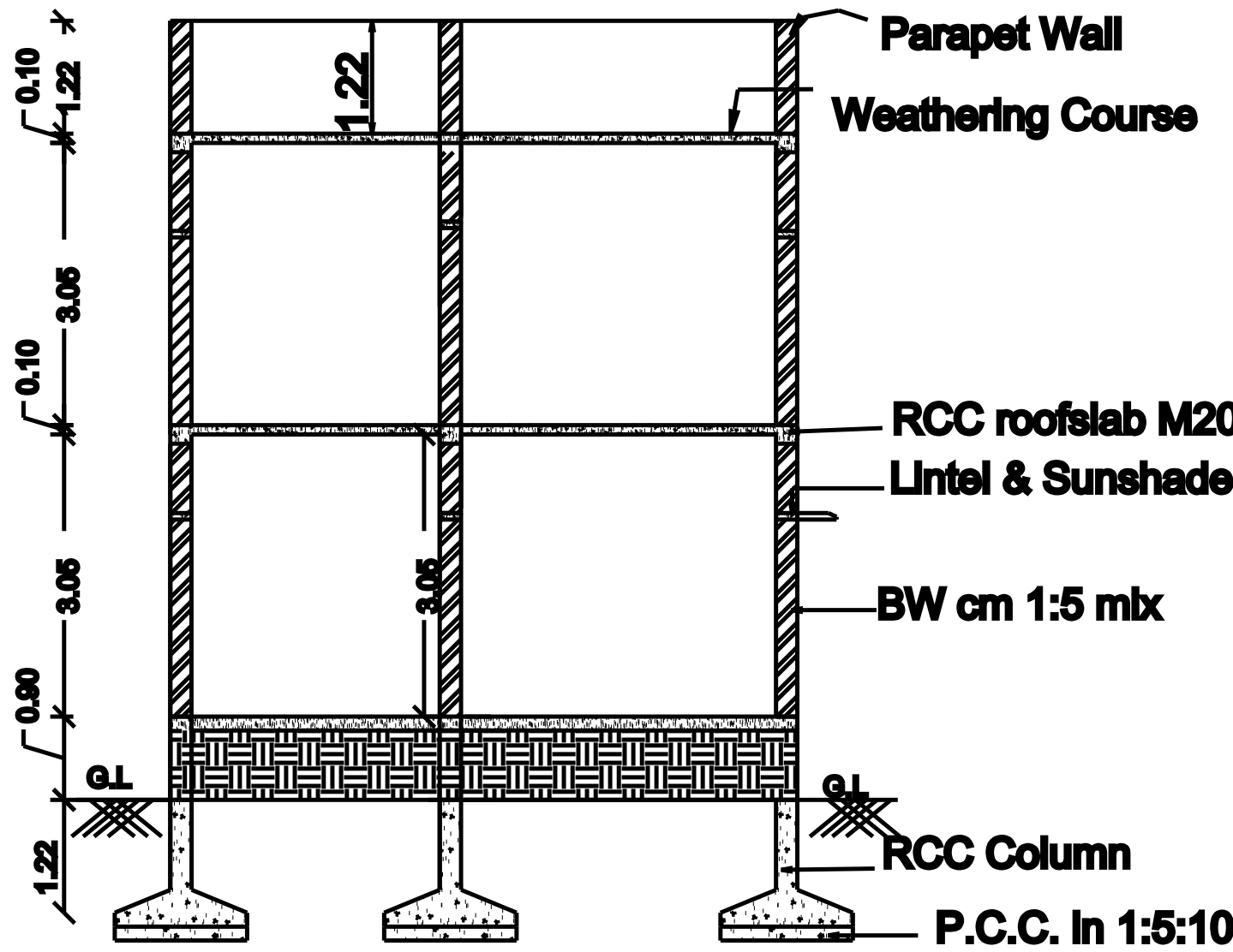
SECTION- BB
