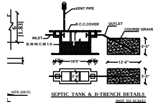
SEPTIC TANK & D-TRENCH DETAILS
