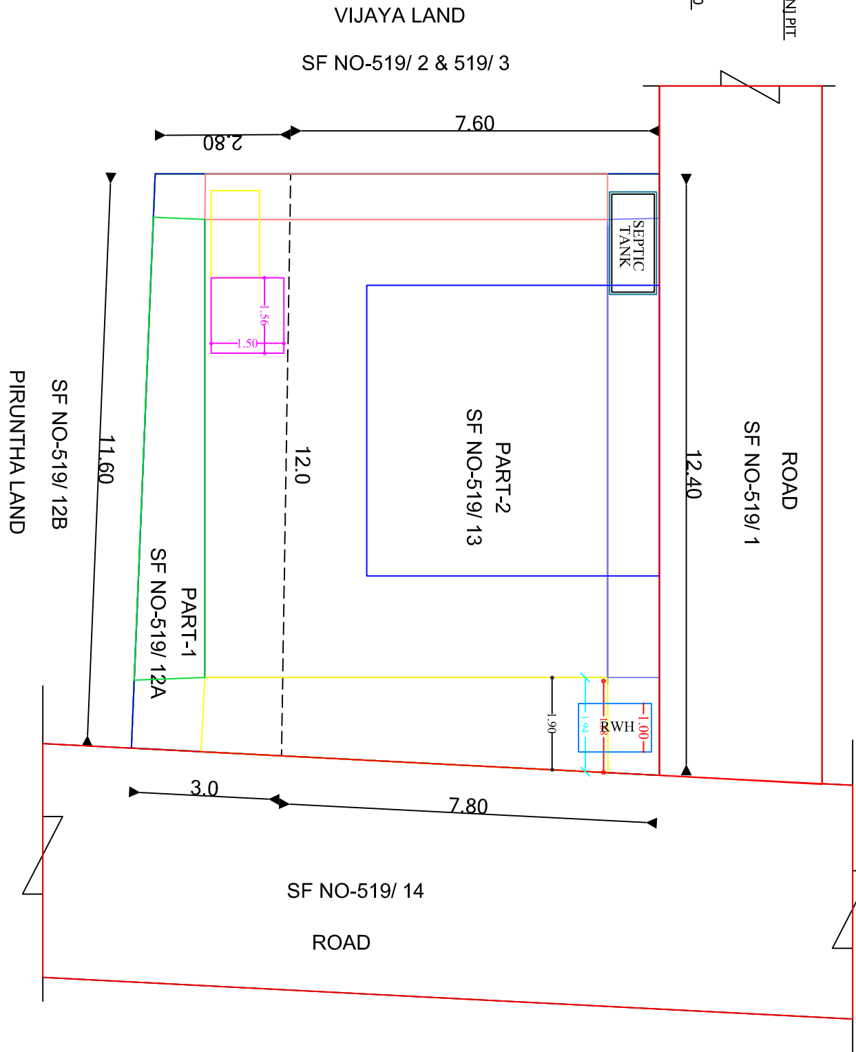
SITE PLAN
