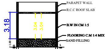
SECTION "AB"
