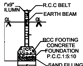
FOUNDATION DETAILS
