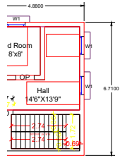
POSED FIRST FLOOR PLAN
