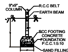
FOUNDATION DETAILS
