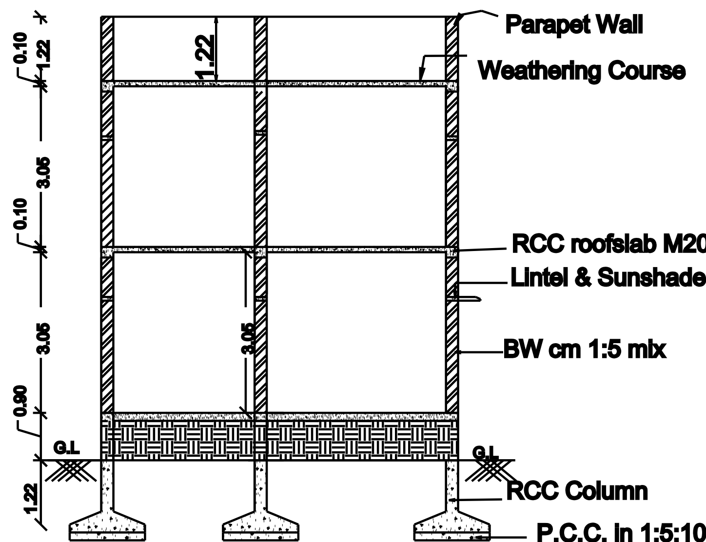
SECTION- BB
