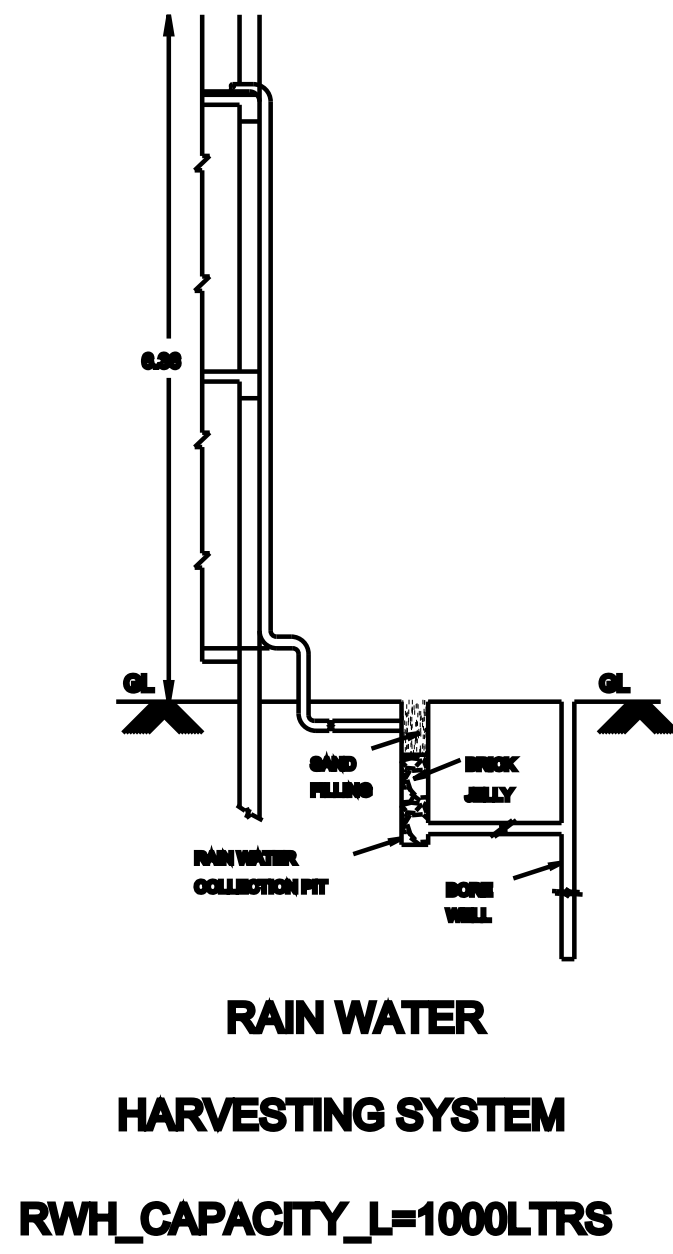
RAIN WATER HARVESTING SYSTEM RWH_CAPACITY_L=1000LTRS
