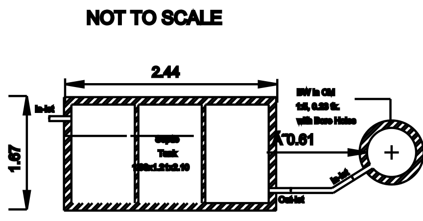
PLAN - SEPTIC TANK & SOAK PIT
