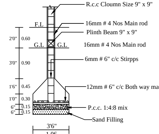
COLUMN DETAILS
