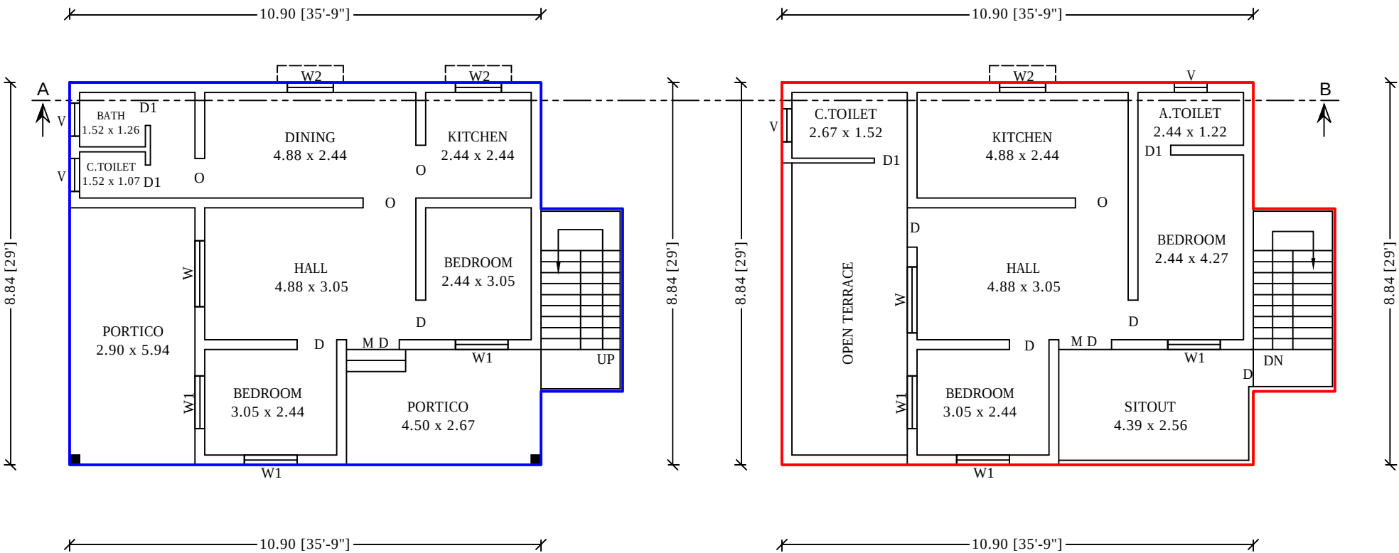
EXI.GROUND FLOOR PLAN
