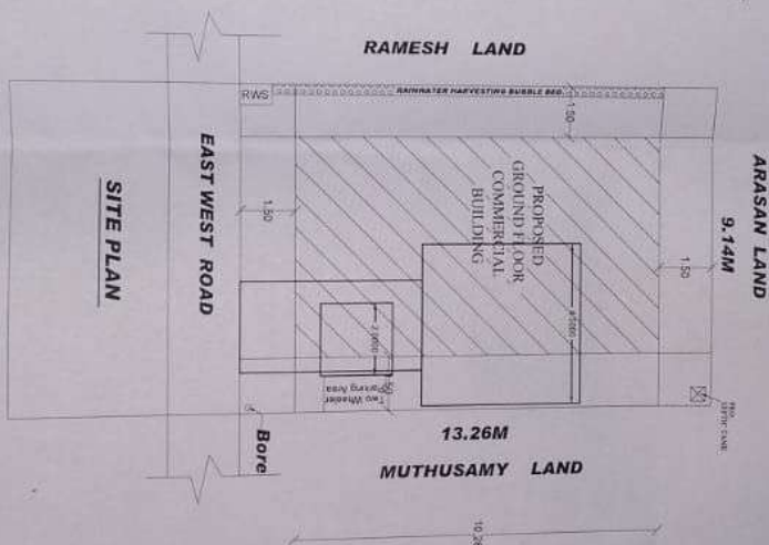
RCC Perforated slab F.S.I = 62.99 / 121.67 = 0.51
