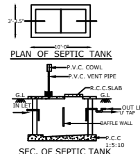
SEC. OF SEPTIC TANK
