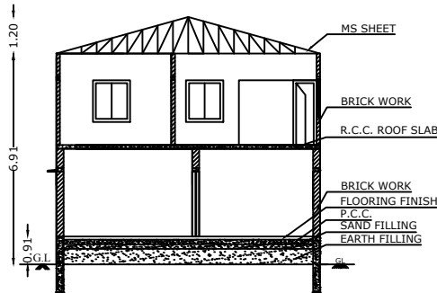
SECTION ON XX
