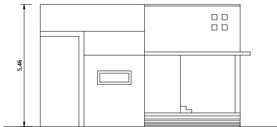
FRONT ELEVATION
