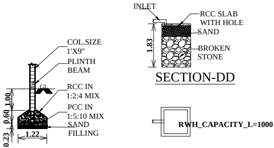
COLUMN DETAILS
