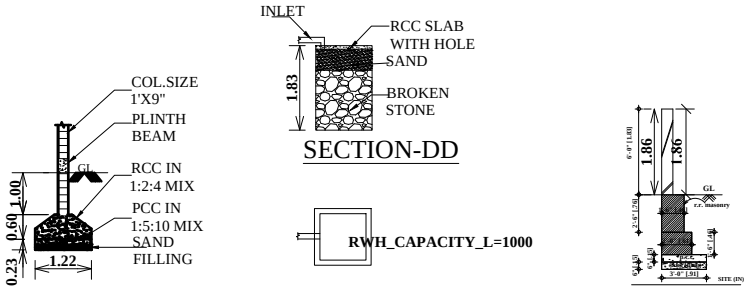
COLUMN DETAILS
