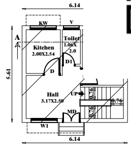
EXT. GROUND FLOOR PLAN
