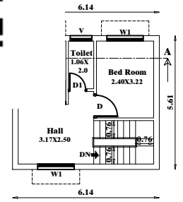
PRO. SECOND FLOOR PLAN
