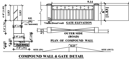
COMPOUND WALL & GATE DETAIL
