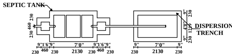
SEPTIC TANK DETAILS.
