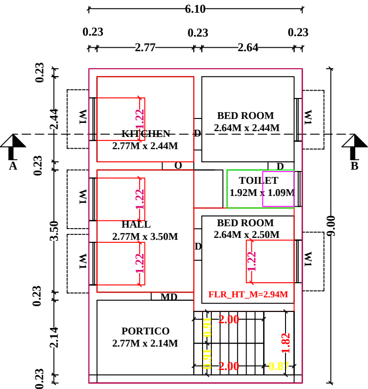
FLOOR-0
