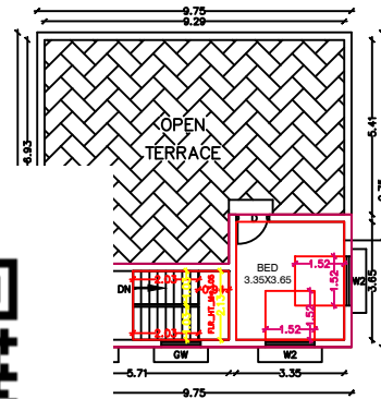
ST FLOOR PLAN
