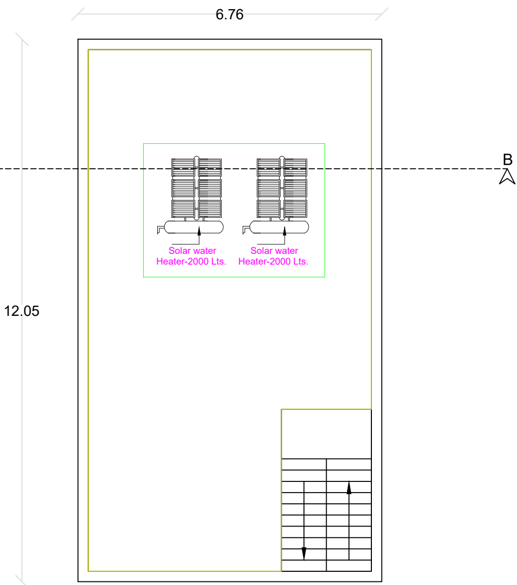
OPEN TERRACE PLAN
