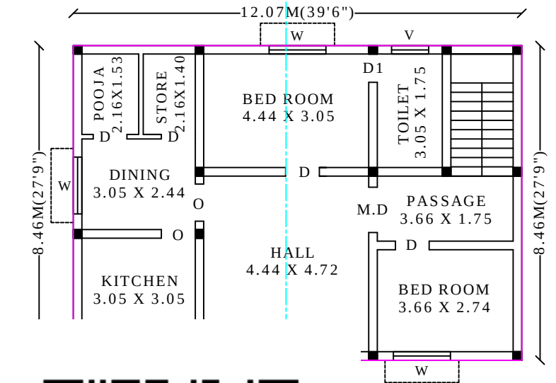
R PLAN
