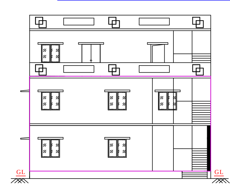
FRONT ELEVATION
