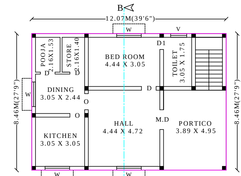
EXG.GROUND FLOOR PLAN
