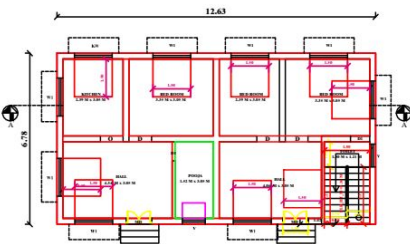
PROPOSED GROUND FLOOR PLAN
