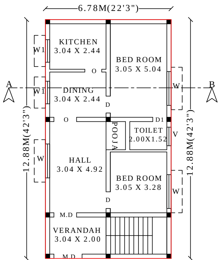
PRO.GROUND FLOOR PLAN (NORTH FACING)
