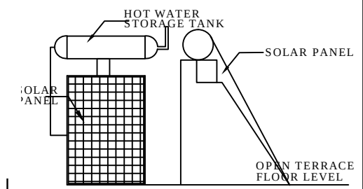
PLAN SIDE ELEVATION SOLAR SYSTEM DETAILS
