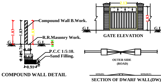
COMPOUND WALL DETAIL SECTION OF DWARF WALL (DW)
