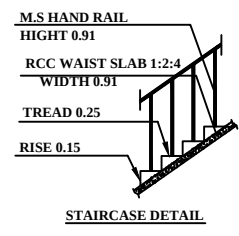
STAIRCASE DETAIL
