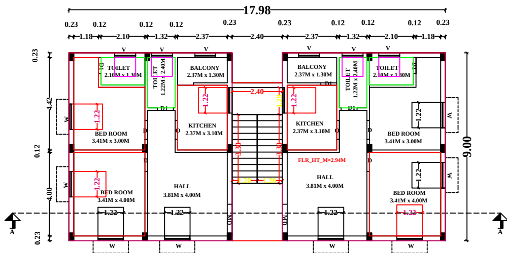
FLOOR-1 PRO.FIRST FLOOR PLAN
