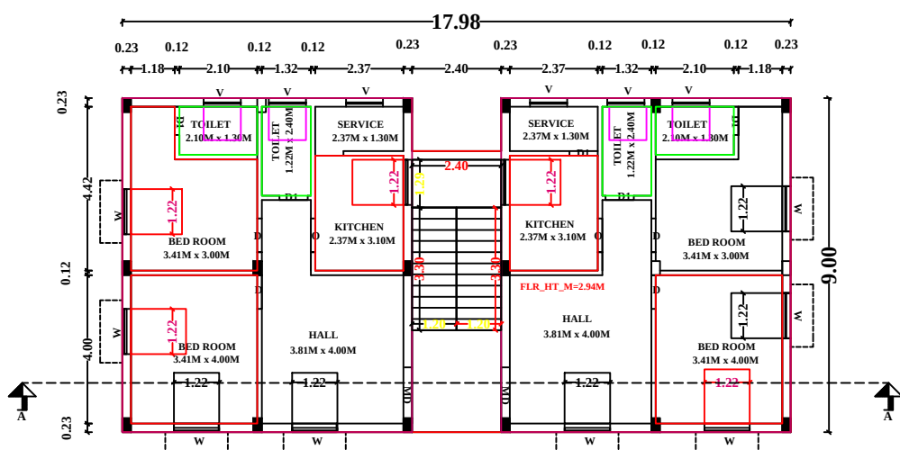
FLOOR-1 PRO.GROUND FLOOR PLAN
