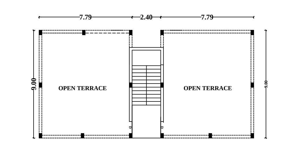
FLOOR-3 PRO.TERRACE FLOOR PLAN
