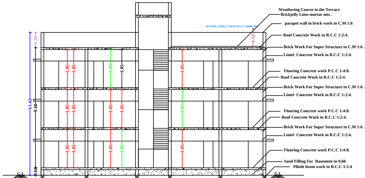
SECTION-AB
