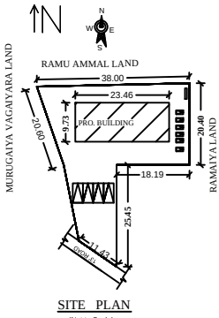
SITE PLAN (Not to Scale)
