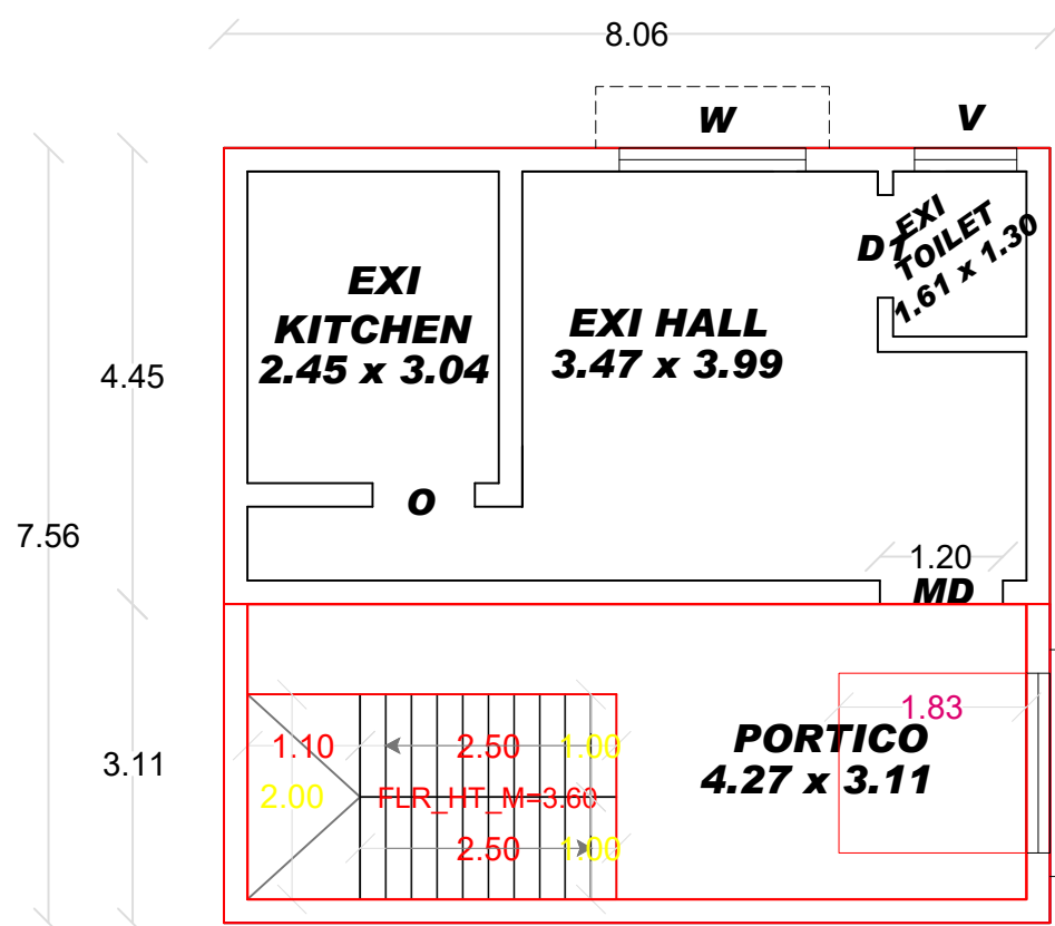
EXISTING AND PROPOSED GROUND FLOOR PLAN
