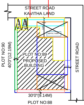
SITE PLAN (Scale = 1 : 1)
