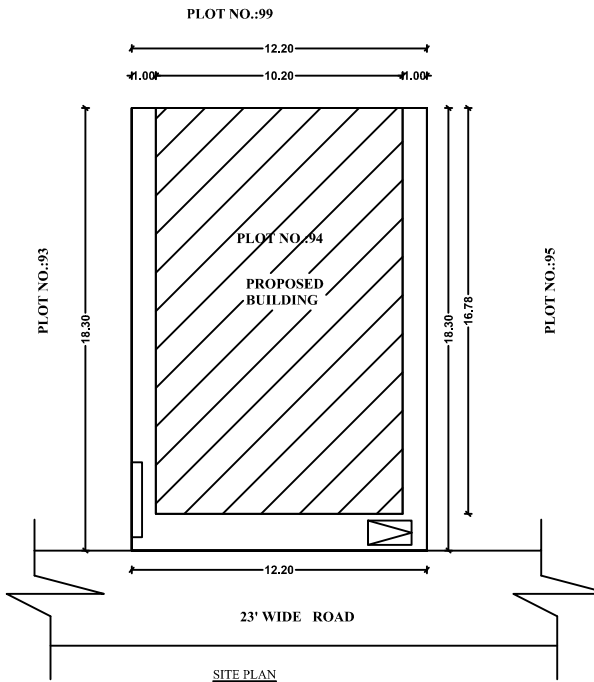
SITE PLAN
