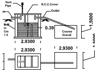
PTIC TANK & D-TRENCH DETAILS
