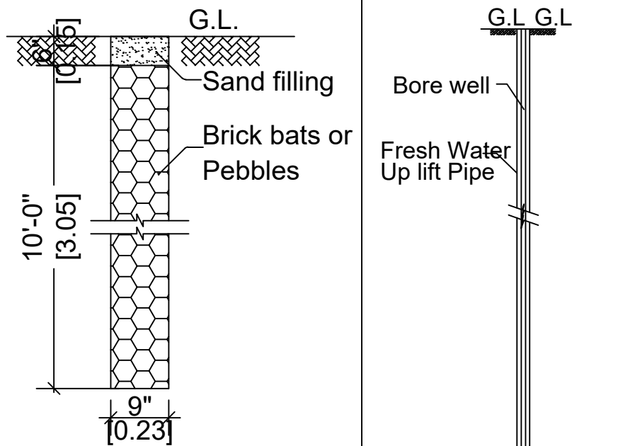
Percolation Pit
