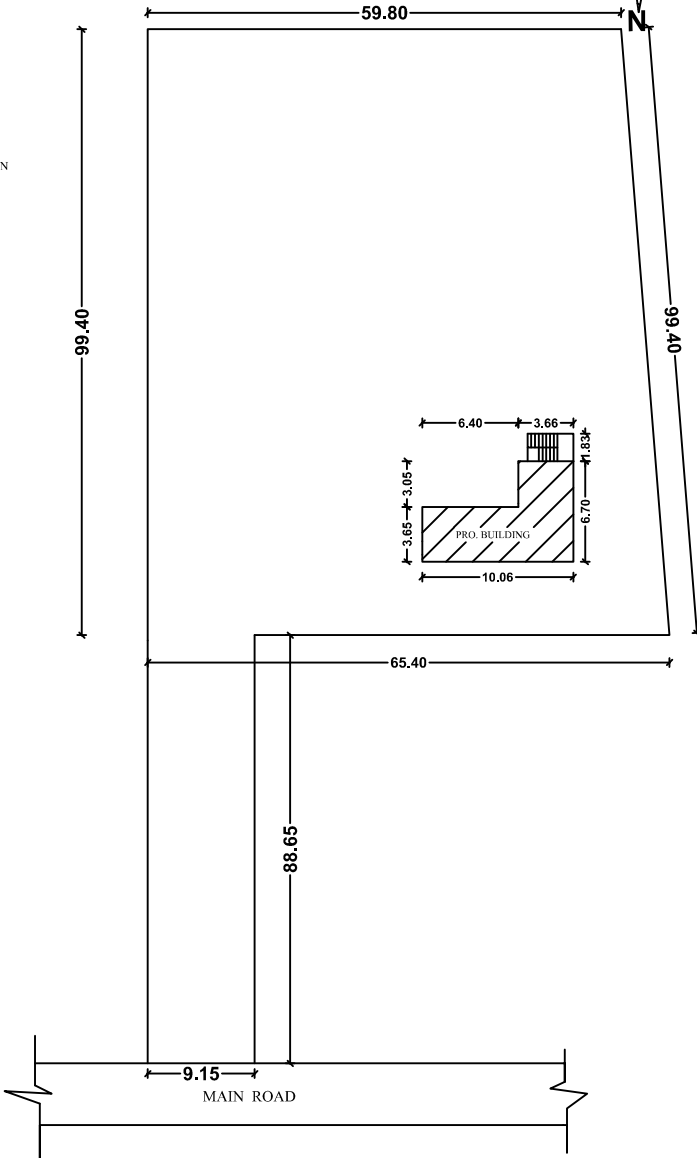
SITE PLAN
