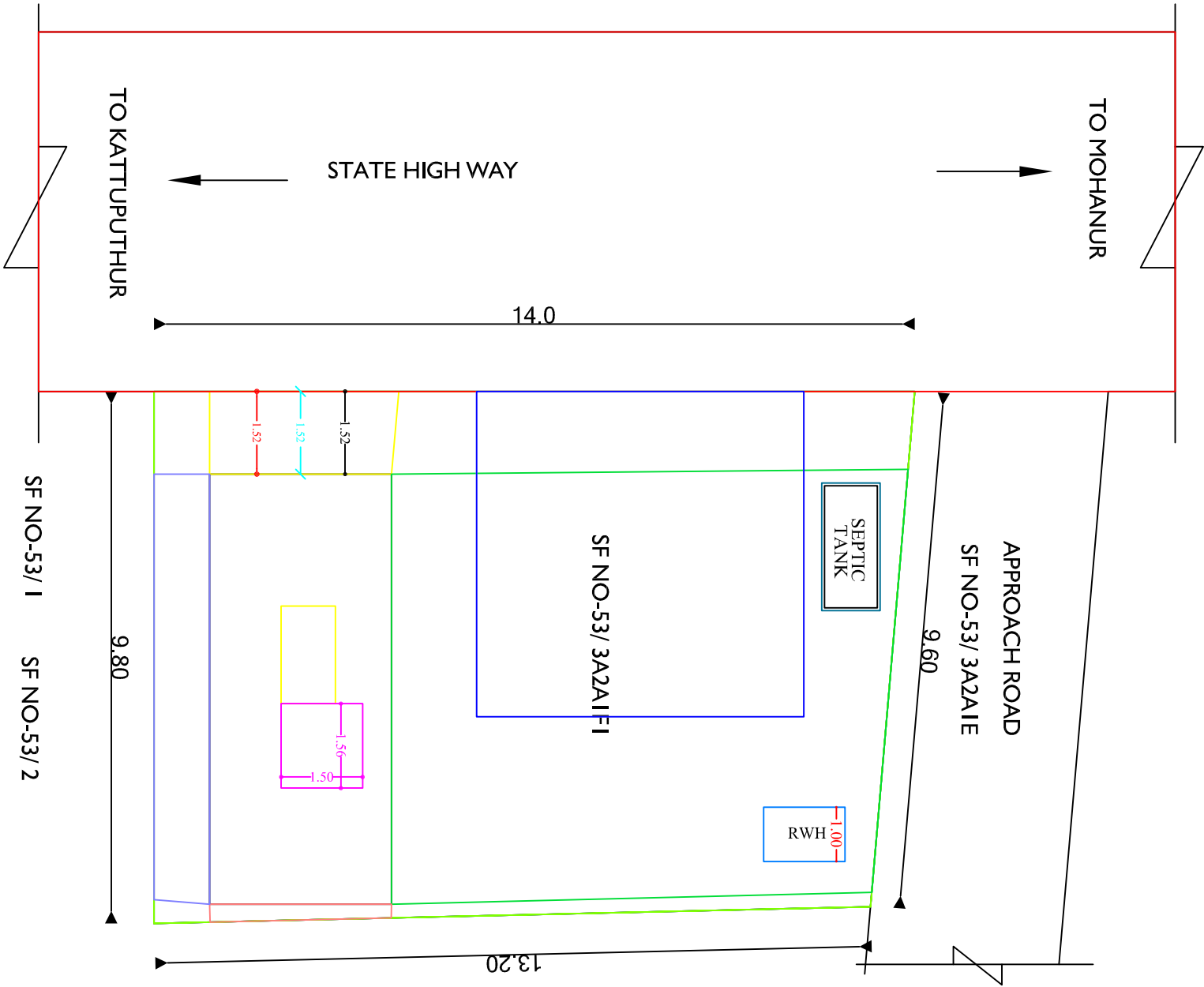
SITE PLAN
