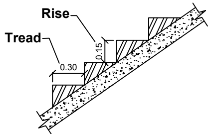
STAIRCASE DETAILS
