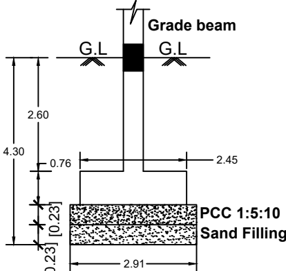
FOUNDATION DETAILS
