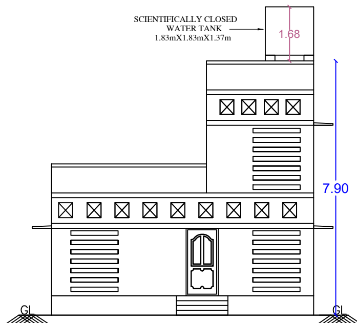
FRONT ELEVATION
