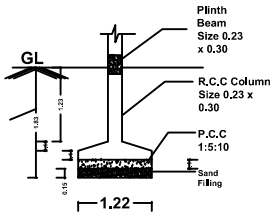
FOUNDATION DETAILS
