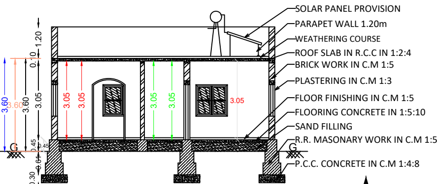
SECTION - XY
