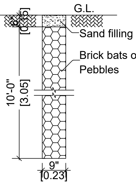
Percolation Pit
