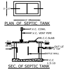
SEC. OF SEPTIC TANK
