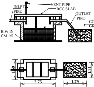
SEPTIC TANK & D-TRENCH DETAILS (NOT TO SCALE)
