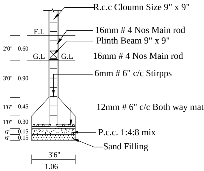
COLUMN DETIAL
