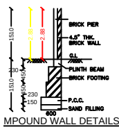
MPOUND WALL DETAILS
