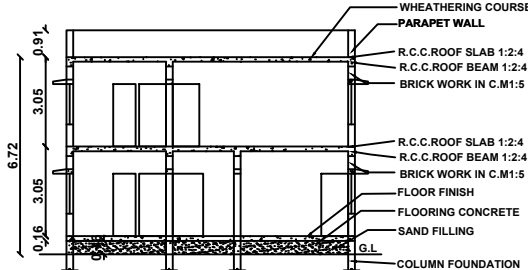
SECTION ON G.G
