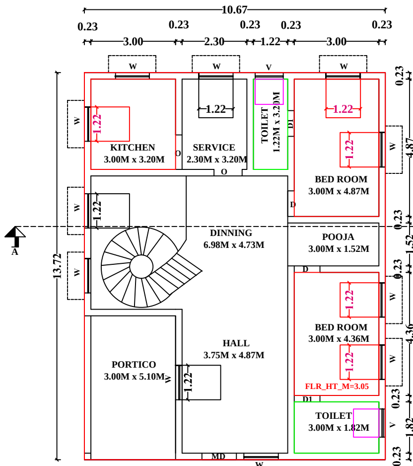
FLOOR-0 PRO.GROUND FLOOR PLAN
