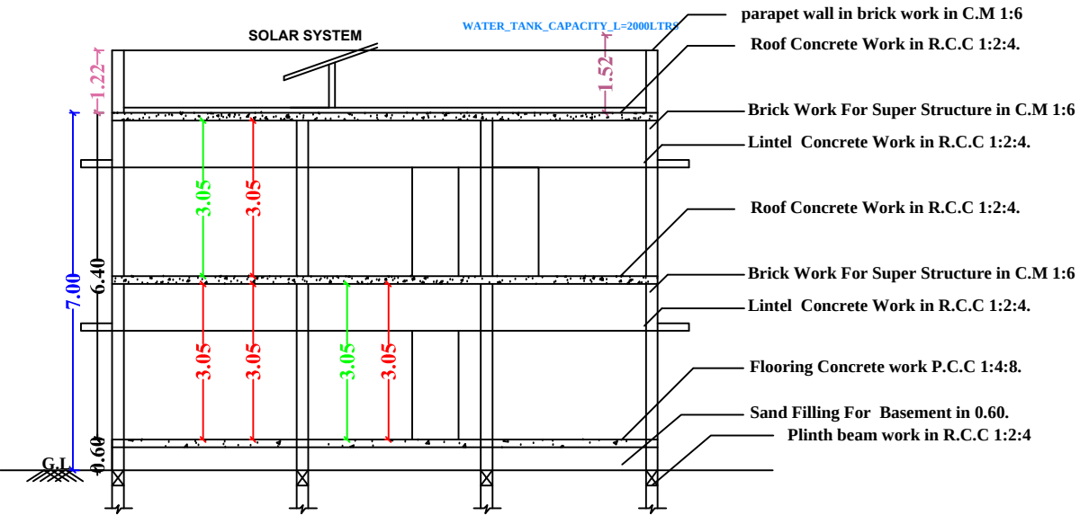
SECTION-AB
