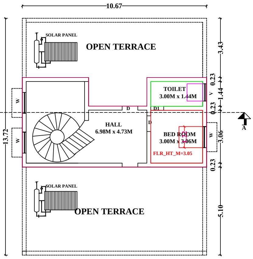
FLOOR-1 PRO.FIRST FLOOR PLAN
