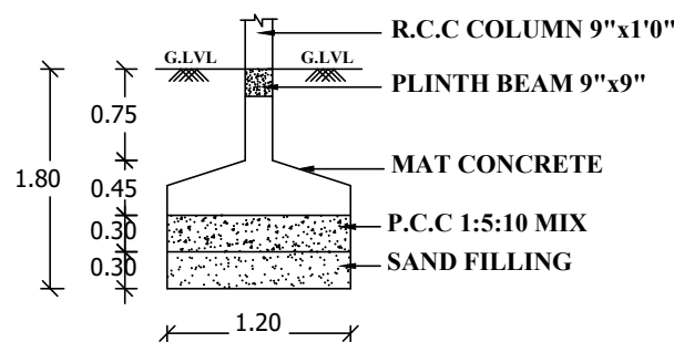
COLUMN FOUNDATION (NOT TO SCALE)
