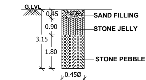
RAIN WATER HARVESTING PIT (NOT TO SCALE)
