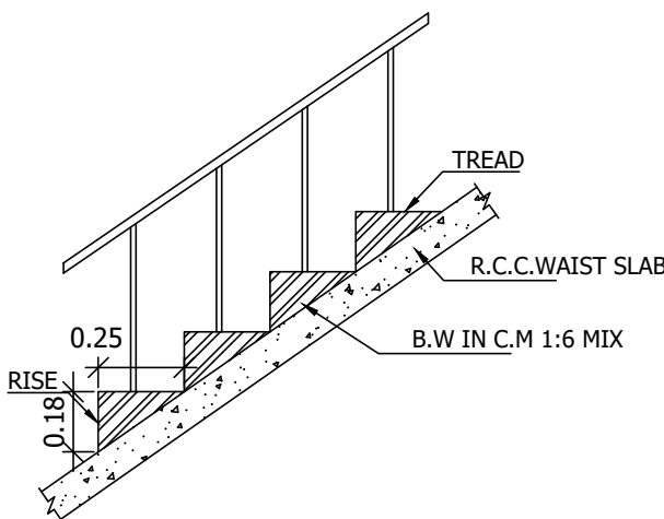
SECTION OF STAIRCASE (NOT TO SCALE)
