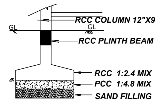
FOUNDATION DETAILS
