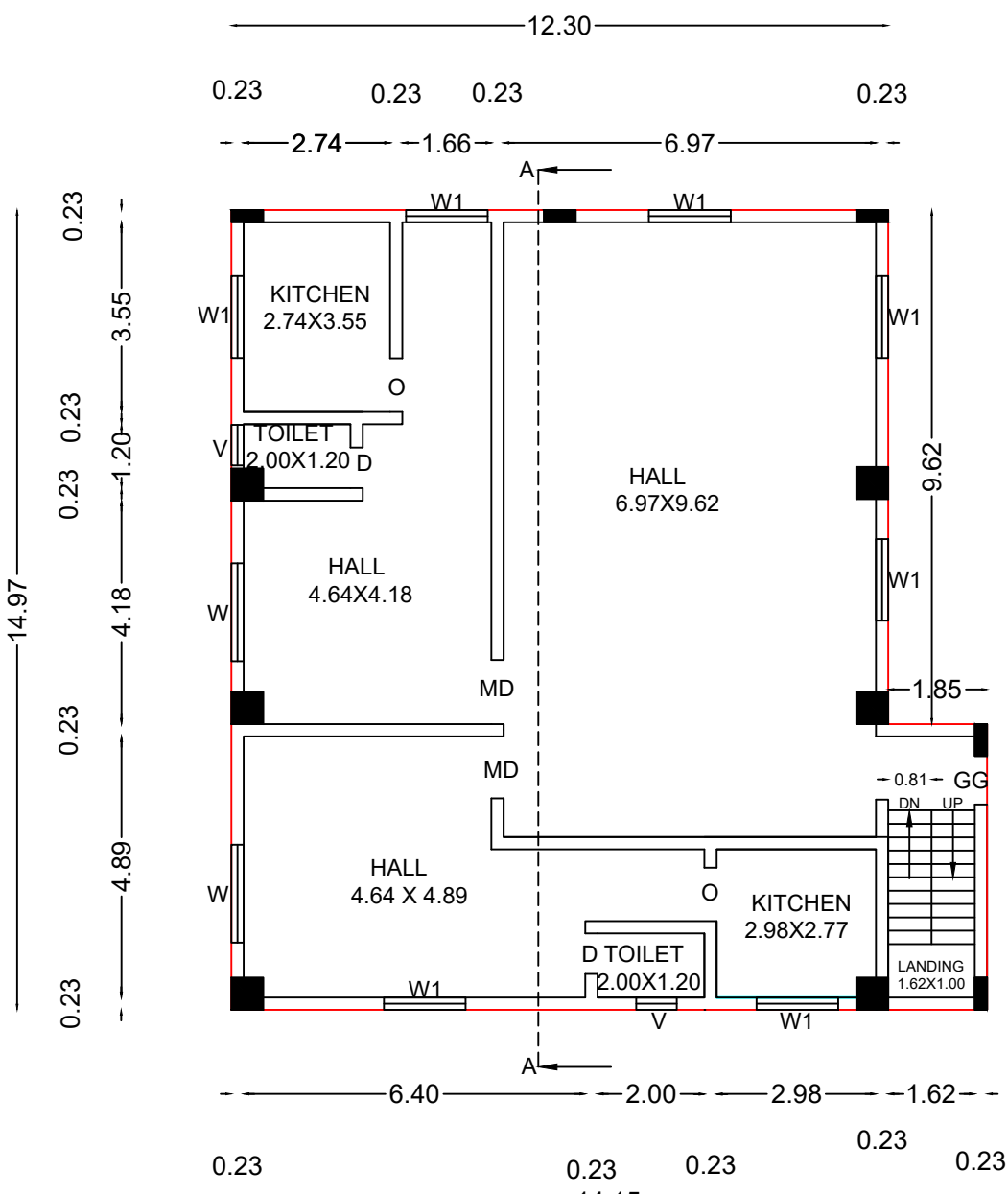
GROUND FLOOR
