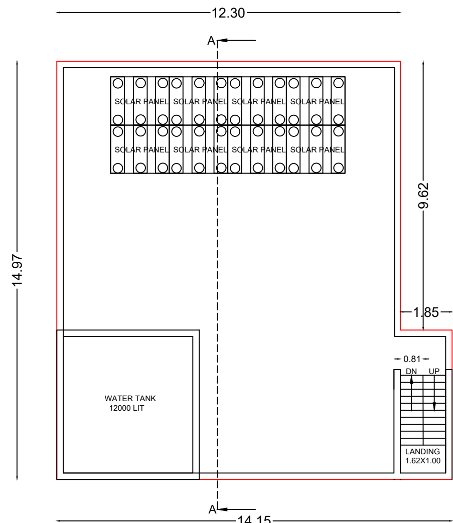
TERRACE FLOOR
