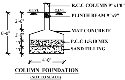
COLUMN FOUNDATION (NOT TO SCALE)
