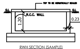
RWH_SECTION (SAMPLE)
