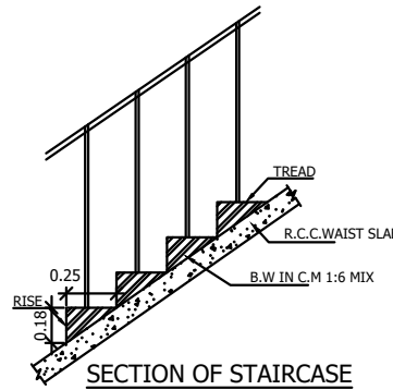
SECTION OF STAIRCASE (NOT TO SCALE)
