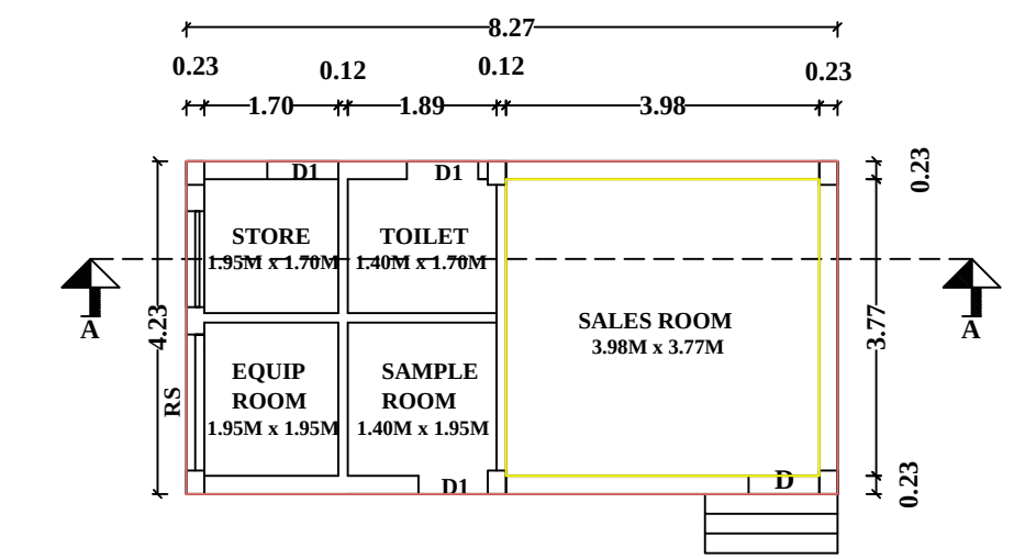
FLOOR-0 PRO.GROUND FLOOR PLAN
