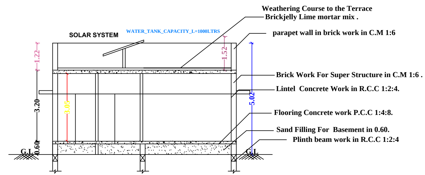
SECTION-AB
